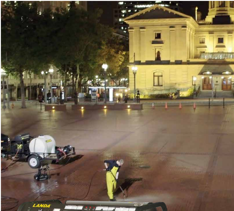
The super-sized PGHW5-50524E model is powered by a water-cooled 27-horsepower Kawasaki engine for extra-high-pressure cleaning power.
